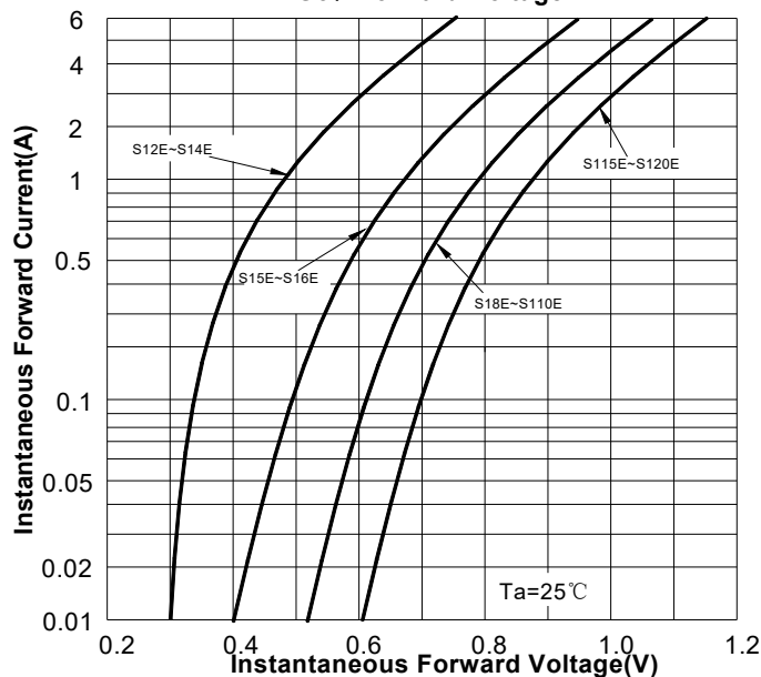
FIG3: Forward Voltage
